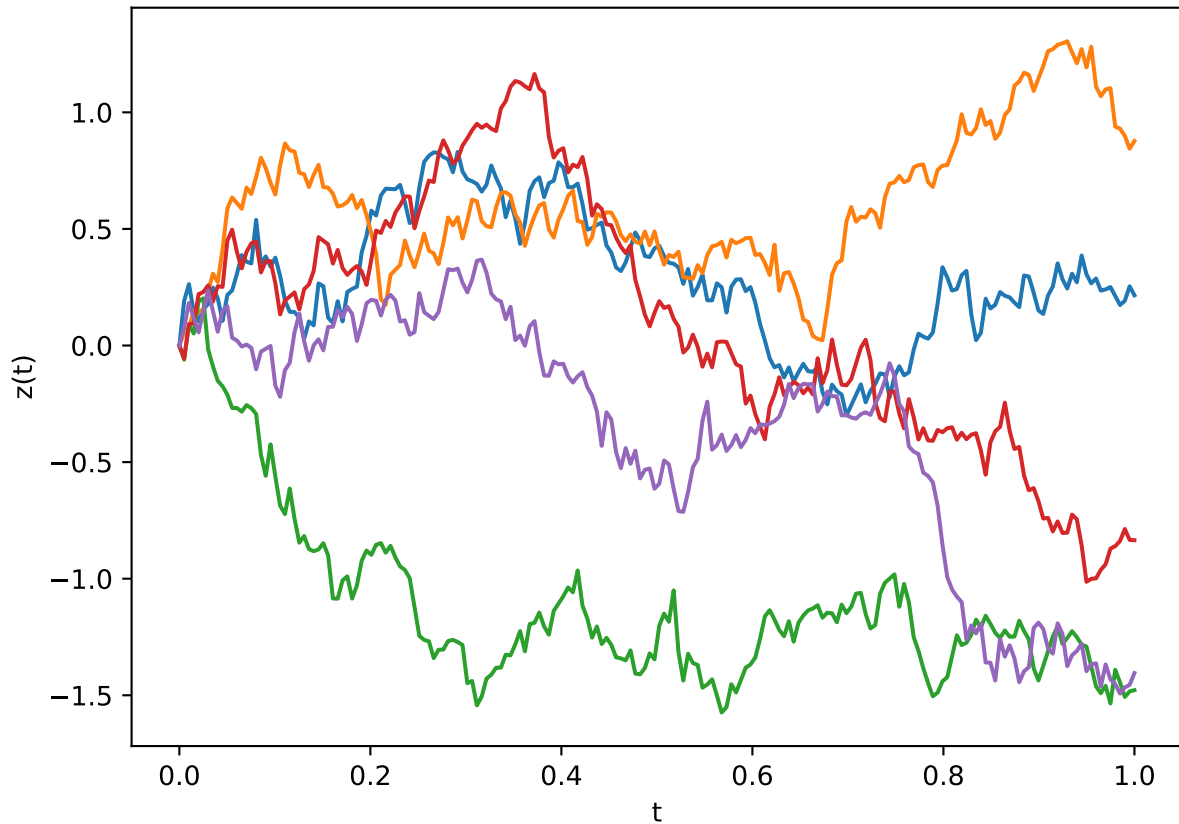
GP - Brownian motion kernel ( \min\{s,t\} )
